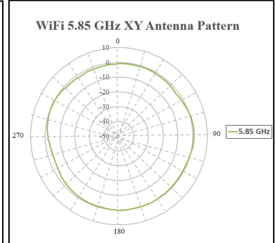
5.85 GHz Plane
