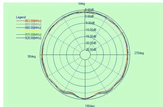
Antenna Radiation Patterns
